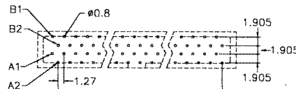
P.C. Board Layout Top View (20,32,40,52,60,68,80,100 Position)
