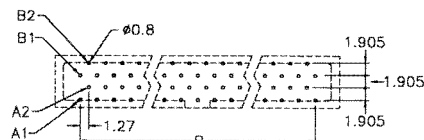
P.C. Board Layout Top View (26,34,50 Position)
